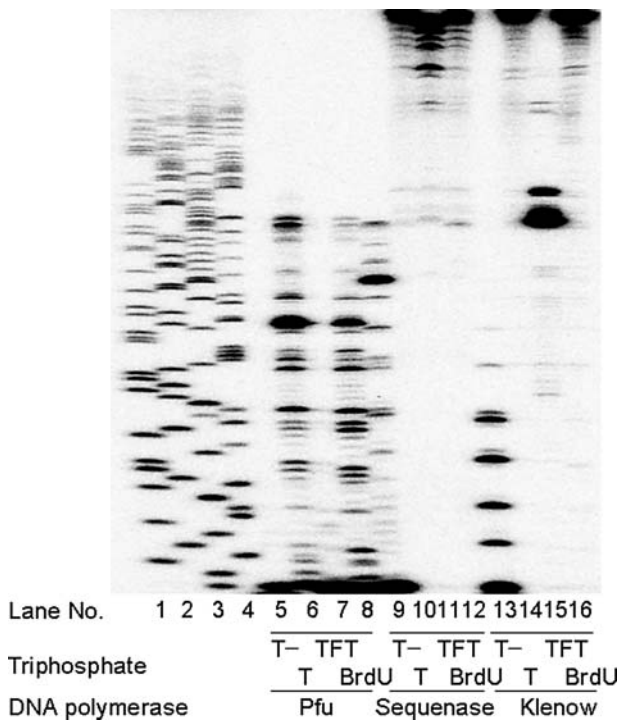
FIGURE 2 Incorporation TFT into DNA by several DNA polymerases. Actions of TFT and BrdU on DNA primer extension in vitro. The ability of pfu DNA polymerase (pfu, 2.5 U/10 \mu L), Sequenase DNA polymerase (Sequenase, 13 U/10 \mu L), and Klenow fragment DNA polymerase (Klenow, 2.0 U/10 \mu L) to extend the 5'- 32 P-labeled primer/M13mp19(+) DNA (5 \mu g/mL) was evaluated in the presence of dATP, dGTP, and dCTP with or without dTTP, with TFT-TP, and with BrdUTP. Lanes 1–4, dideoxynucleotide sequencing of the M13mp19(+) DNA template with ddGTP, ddATP, ddTTP, and ddCTP, respectively, are indicated.
